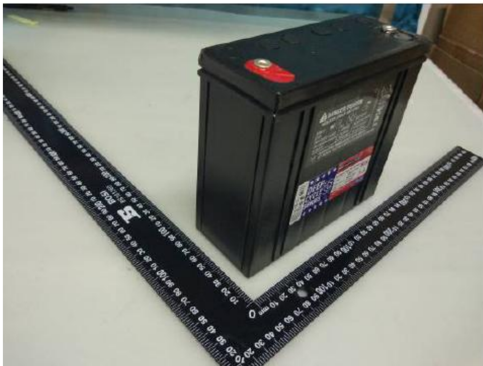
Photo 4 ( C&D DCS-18UNC RIT 12V 18Ah)
